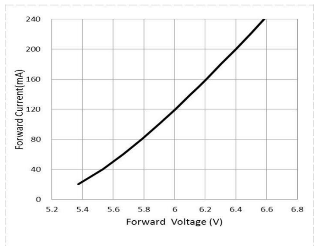
Fig 6. Forward Current vs. Forward Voltage, Tj = 25°C
