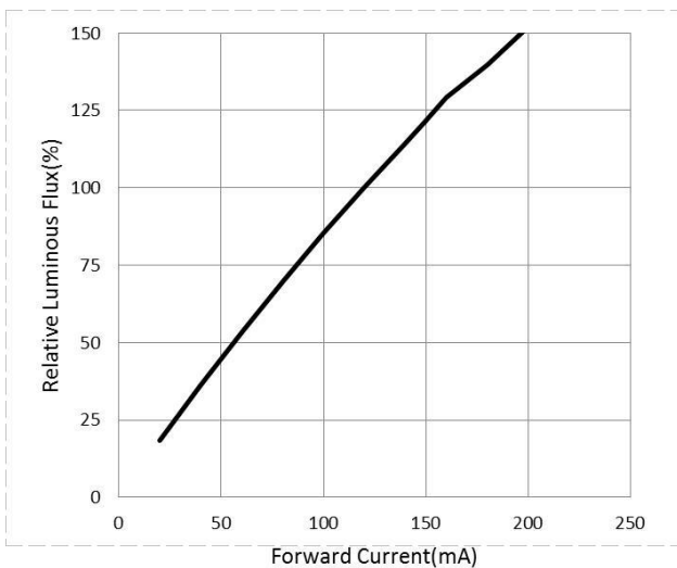
Fig 5. Forward Current vs. Relative Intensity, Tj = 25°C
